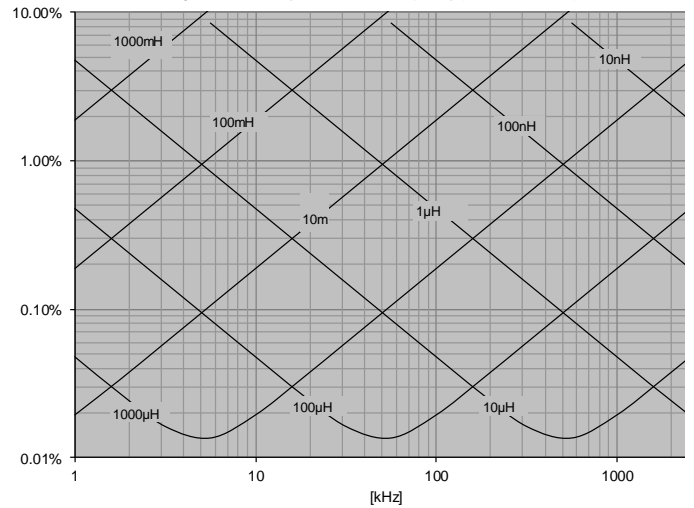
Figure 4: Inductivity Error versus Frequency (Model 2097k-33)
