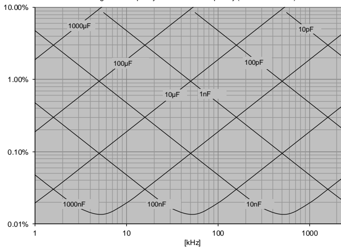
Figure 3: Capacity Error versus Frequency (Model 2097k-33)
