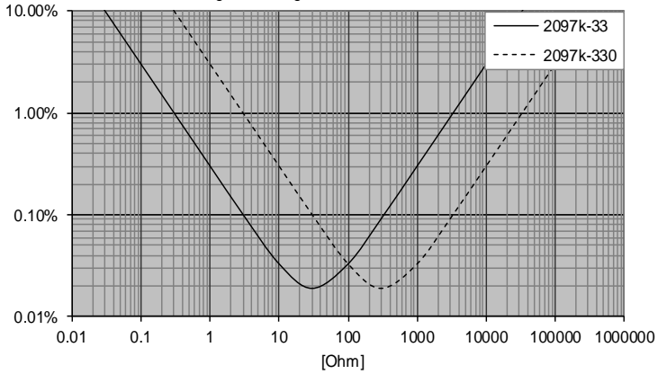
Figure 1: Magnitude Error versus Load
