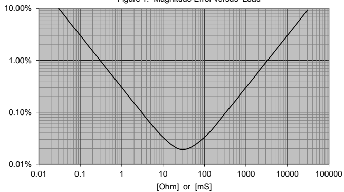
Figure 1: Magnitude Error versus Load
