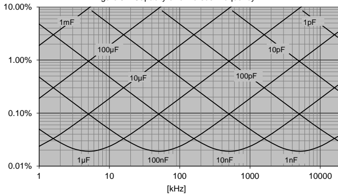
Figure 3: Capacity error versus Frequency
