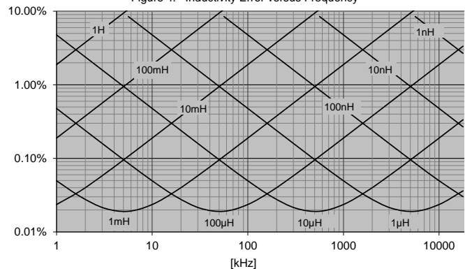
Figure 4: Inductivity Error versus Frequency
