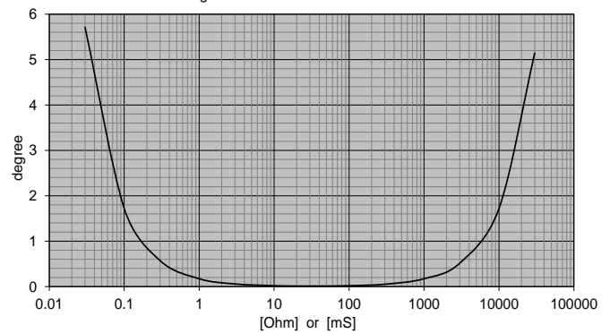
Figure 2: Phase Error versus Load
