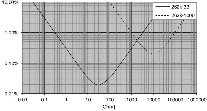
Figure 1: Magnitude Error versus Load
