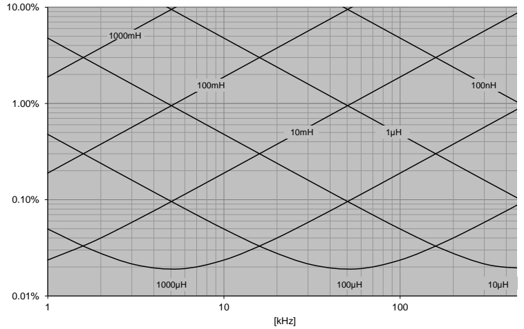
Figure 4: Inductivity Error versus Frequency (Model 262k-33)
